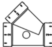
45 Wye
