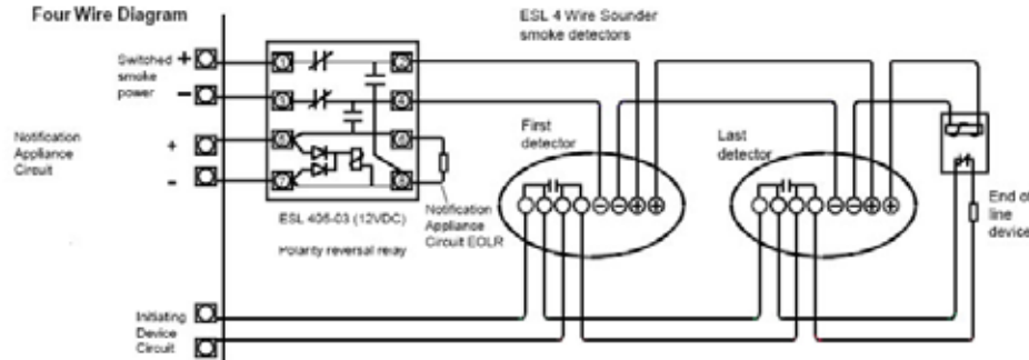
Four Wire Diagram
