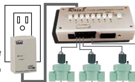
Rain8upb Pro connected to valves with UPB PIM plugged into an outlet.
