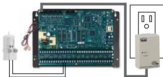
GH502 connected to a zone on an HAI with UPB PIM plugged into an outlet.
